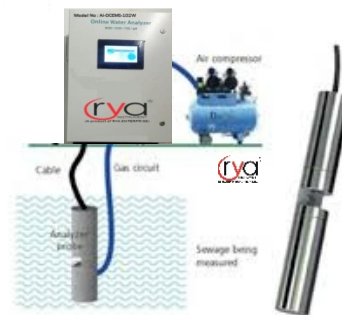
Online effluent monitoring system
