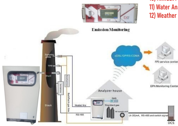
Online Continuous Emission Monitoring system
